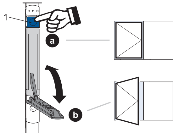
Function test turn double sash window
