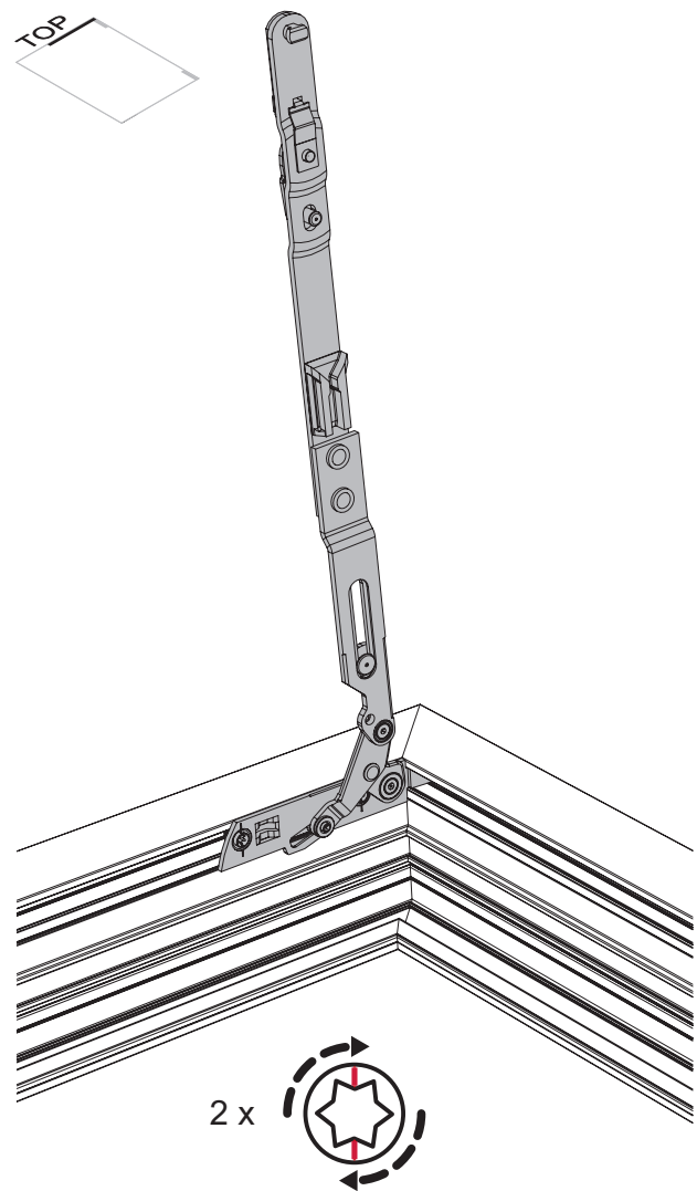
Mounting the shear
