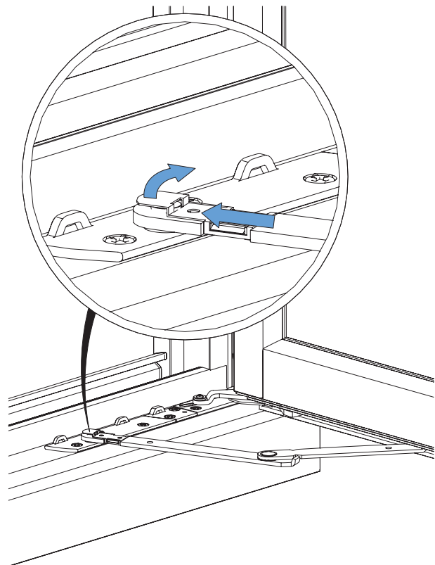
Detaching the turn limiter
